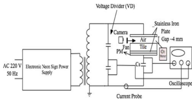
Fig.2 The scheme of DBD test
