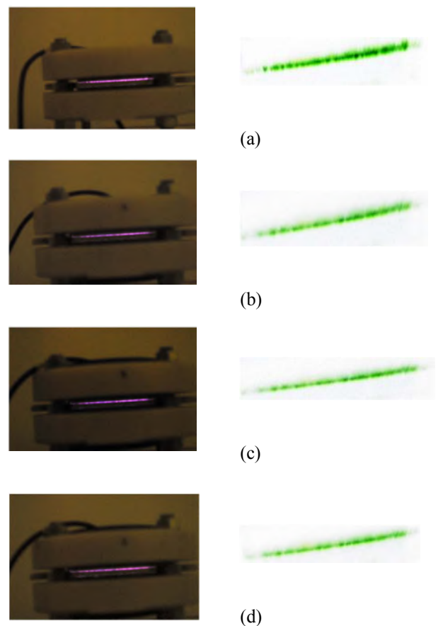
Fig. 4 Plasma Photographs (left side is the real colors and right side is the inverting colors). (a) Model I, (b) Model II, (c) Model III, (d) Model IV.
