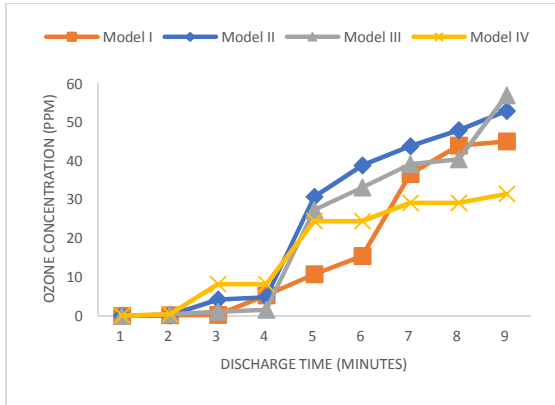
Fig.7 Ozone production for all models.
