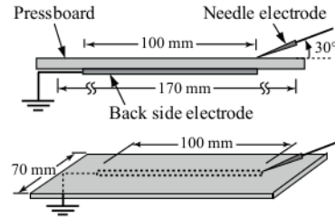
Figure 1. Schematic of electrode system.
