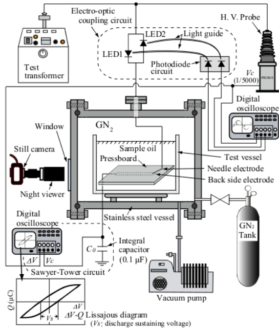
Figure 2. Schematic of experimental setup.
