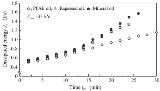
Figure 6. Energy dissipated by creeping discharges.
