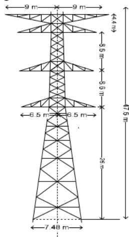
Fig. 5 Characteristic of T/L 275 kV
