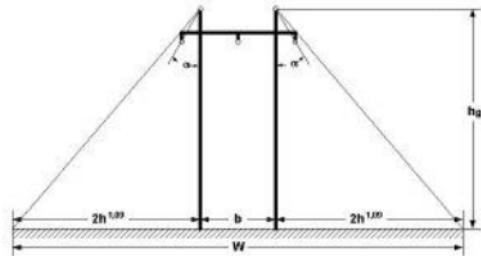
.Fig 3. Illustration of tower
