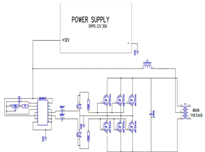
Figure 3. High voltage electronics circuit
