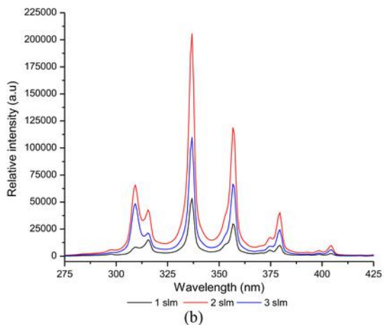
Fig. 2. Optical emission spectroscopy (OES) evaluation of an atmospheric plasma jet near 10mm under the nozzle of the plasma jet reactor (without mice) with various gas flow rates (1, 2 and 3 slm). OH and nitrogen-based reactive species were detected. (a) OES evaluation between 200 nm and 850 nm; (b) OES evaluation between 275 nm and 425 nm.
